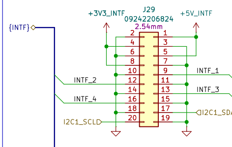
Backplane interface connector
