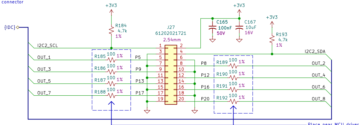
Valve connector
