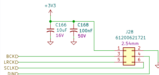
Audio DAC connector
